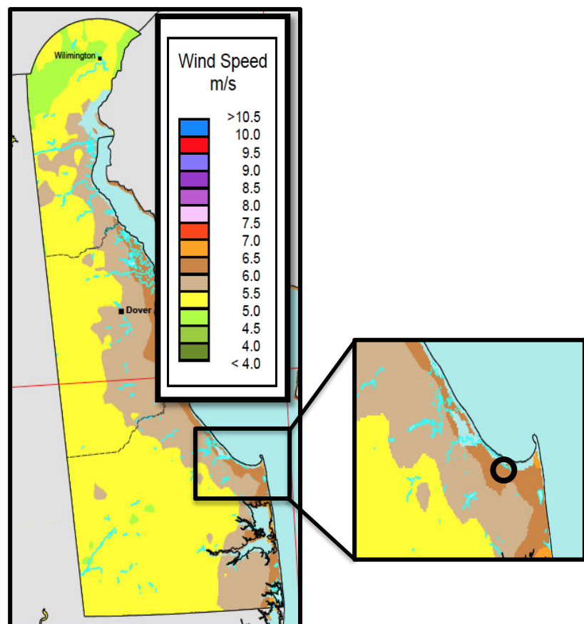
Figure 2. Delaware Average Annual Wind Speeds (80 Meters)
