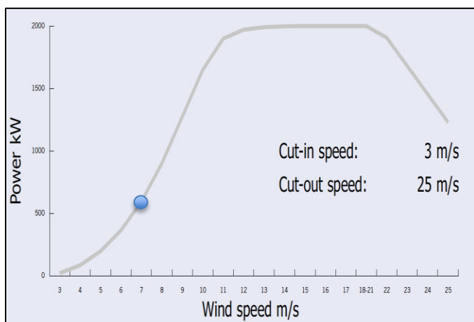
Figure 3. Gamesa G90-2.0 MW Power Curve
