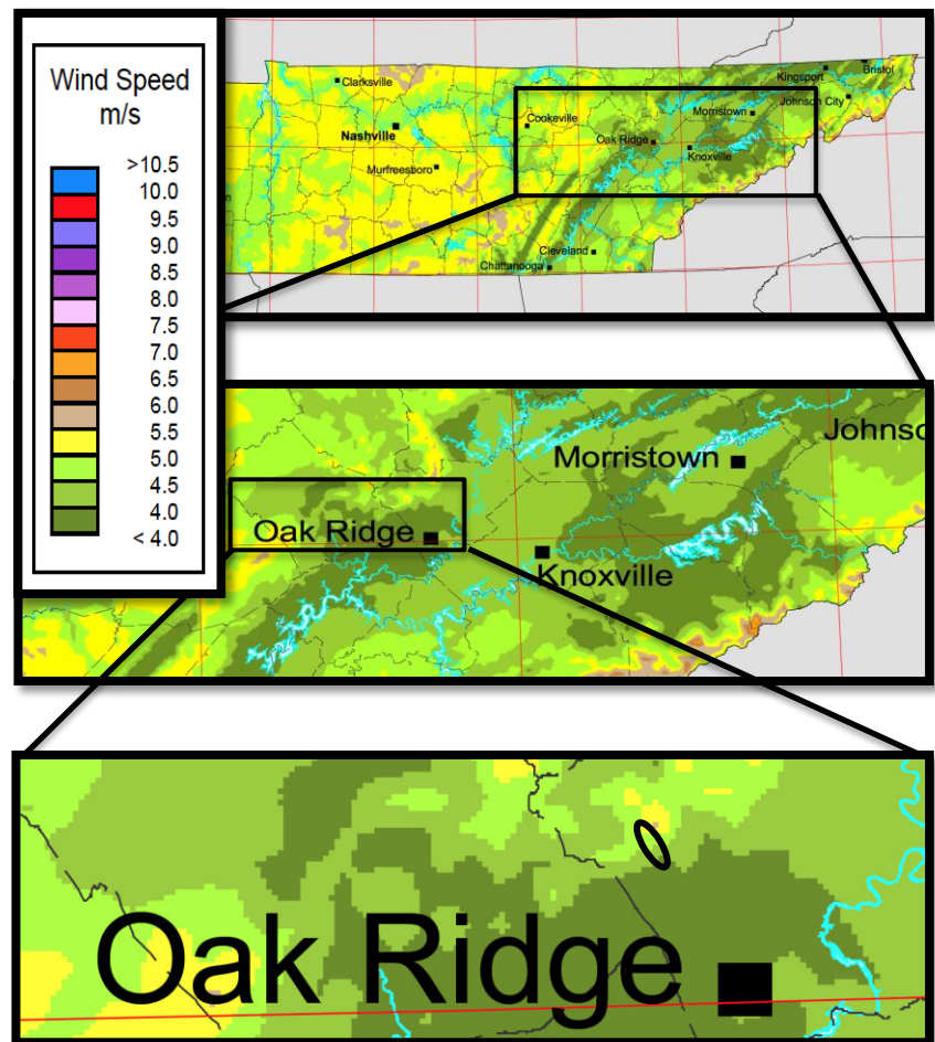
Figure 1. Tennessee Average Annual Wind Speeds (80 Meters)
